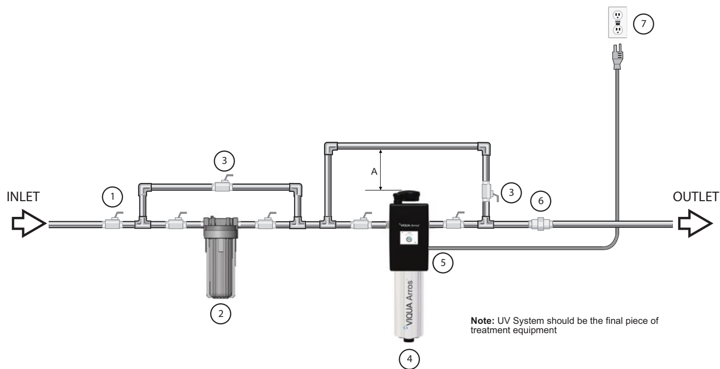
Figure 3 UV System
